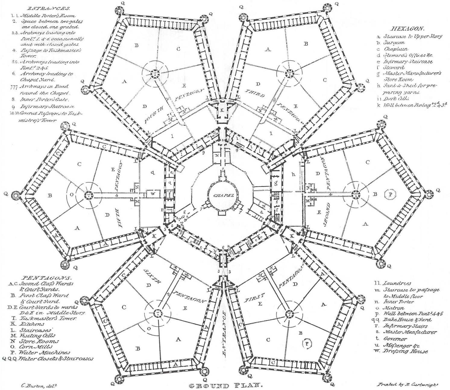
Figure 7.1.1: Millbank Prison Plan 1828 (opened in 1816, closed in 1890)
