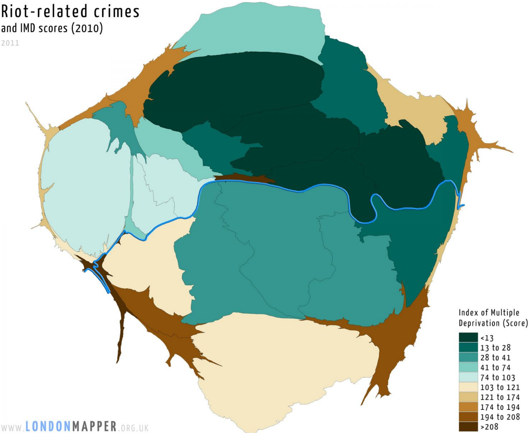
Figure 2.3.2: Riot-related crimes and Index of Multiple Deprivation score, London 2010
